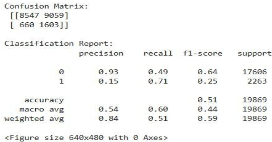
Figure 6: Confusion Matrix and Classification Report
